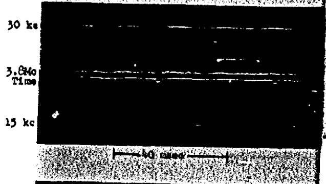
Fig. 3.61 Narrow-band responses Shot No. 2 1000 km from ground zero
